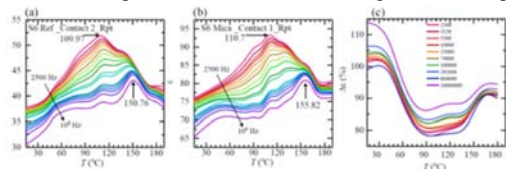
(a) Dielectric constant of heterostructure sample of PVDF/MMA/PVDF layers, (b) Dielectric constant of heterostructure sample of PVDF/layered Mica-MMA/PVDF layers and (c) Display the calculated enhanced dielectric constant of sample at (b) due to intercalated Mica layers.
